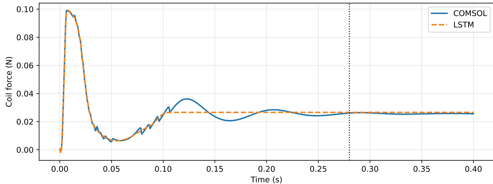
Force Prediction, Test RMSE = 0.0009095 N, R2 = -6.7604
