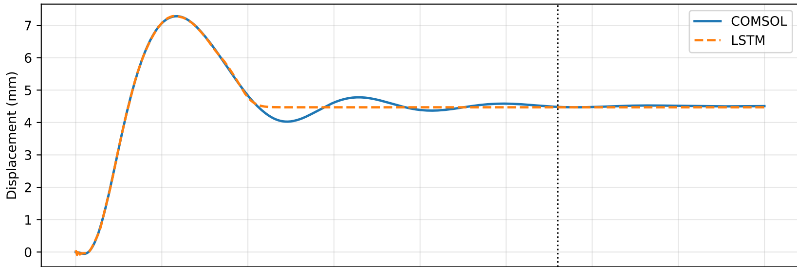
Displacement Prediction, Test RMSE = 0.03609 mm, R2 = -3.6697
