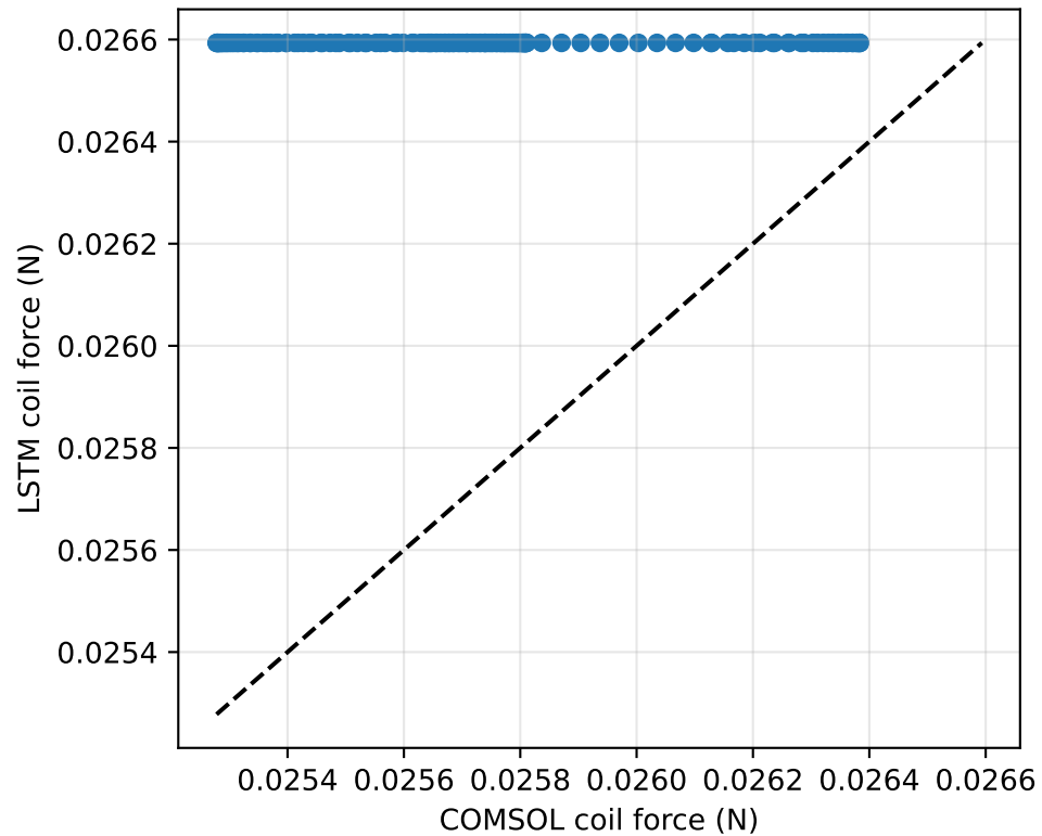
Force parity, R^2 = -6.7604
