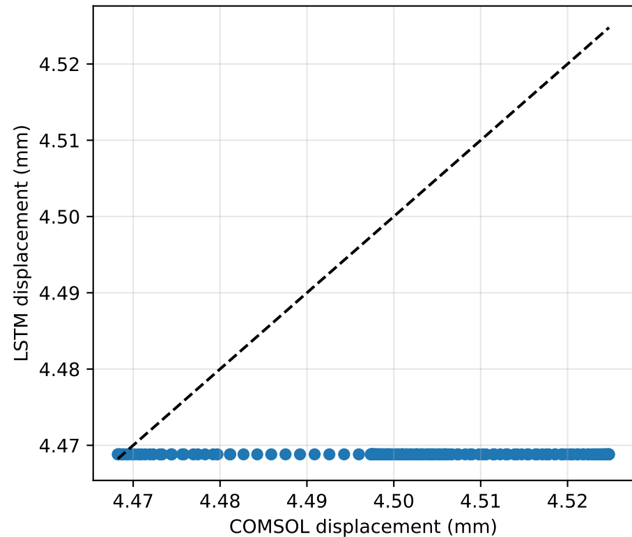
Displacement parity, R^2 = -3.6697
