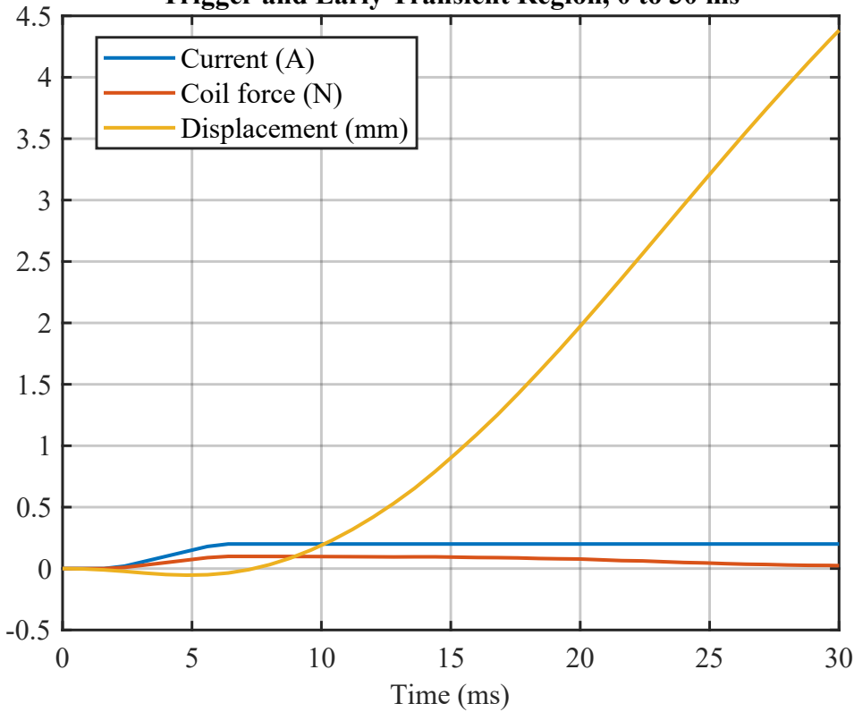
Trigger and Early Transient Region, 0 to 30 ms
