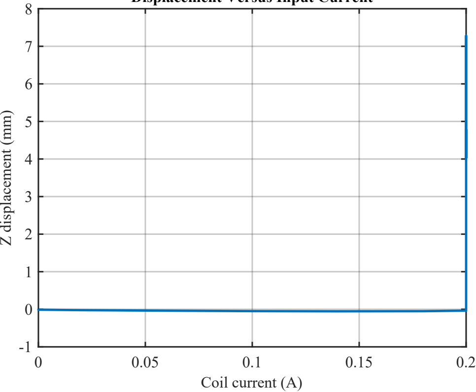
Displacement Versus Input Current
