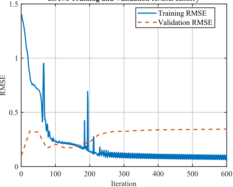
LSTM Training and Validation RMSE History
