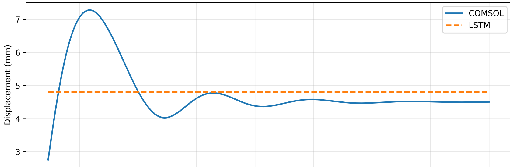
Displacement Prediction, test RMSE = 0.9571 mm, R2 = -0.0225
