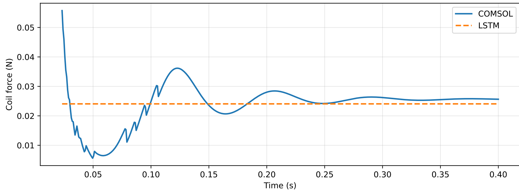
Force Prediction, test RMSE = 0.00788 N, R2 = -0.0345
