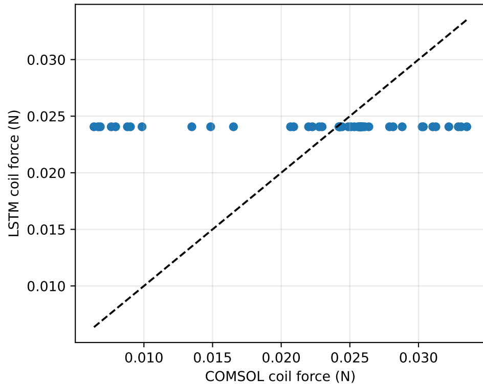
Force parity, R^2 = -0.0345
