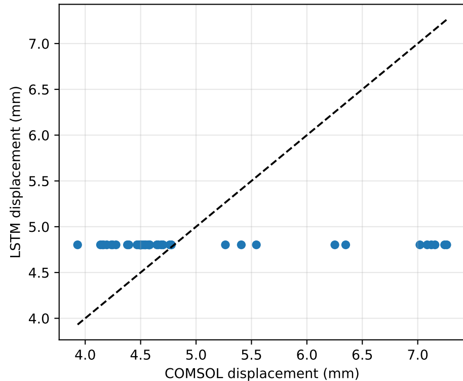
Displacement parity, R^2 = -0.0225
