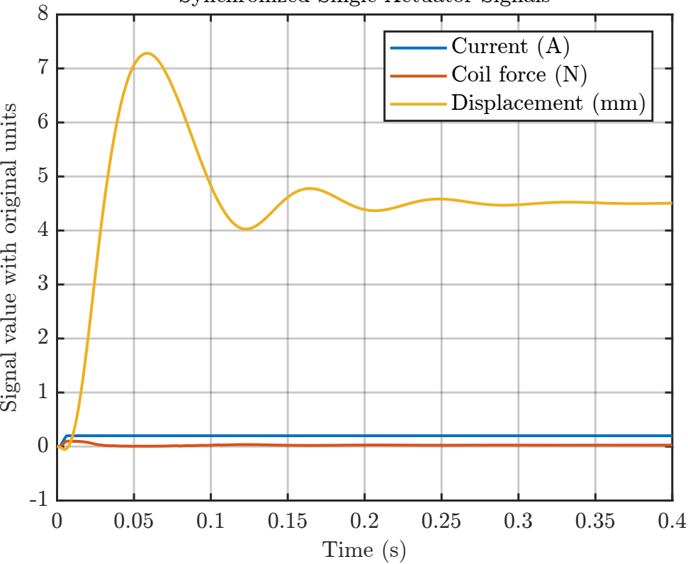
Synchronized Single Actuator Signals
