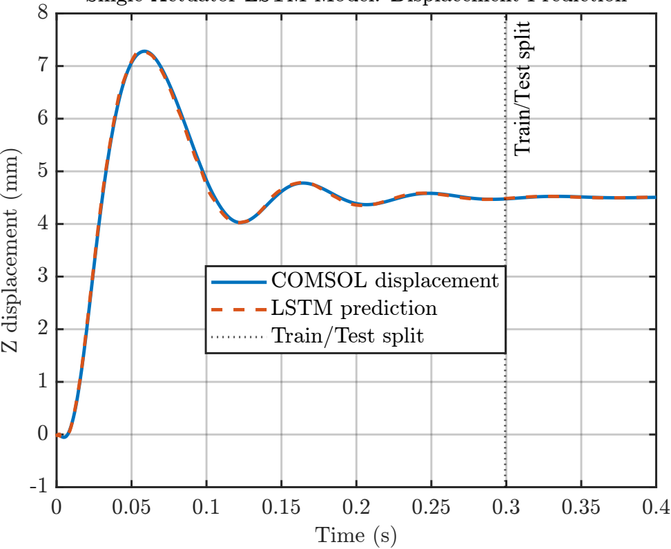
Single Actuator LSTM Model: Displacement Prediction
