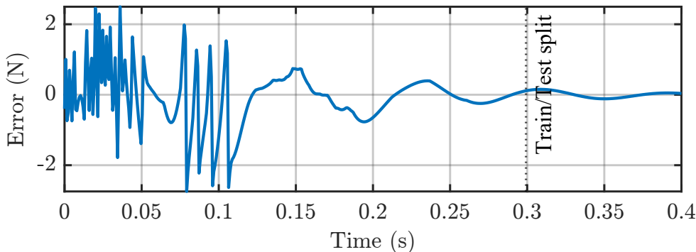
\times 10^{-3} Coil Force Prediction Error: COMSOL minus LSTM
