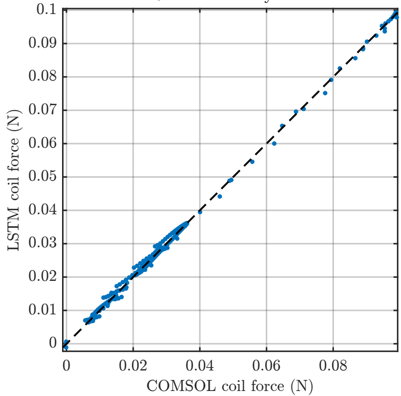
Coil Force Parity Plot
