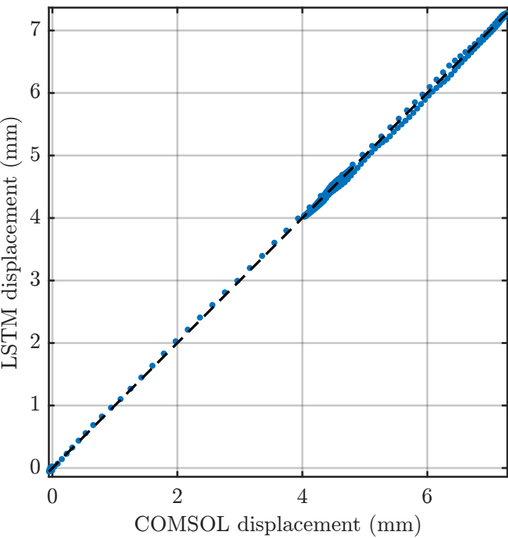
Displacement Parity Plot
