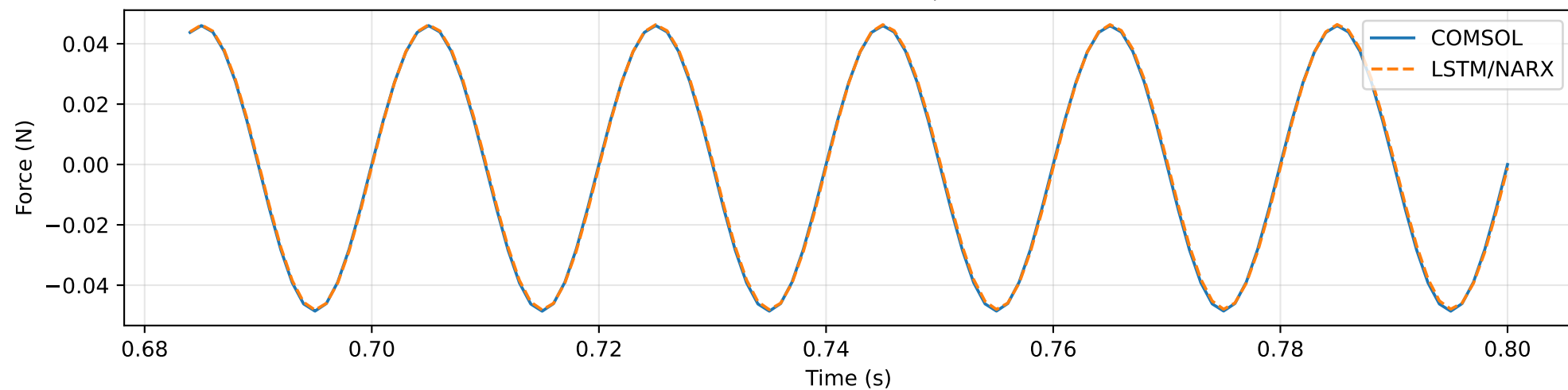
Force: RMSE=0.000765 N, R2=0.9995
