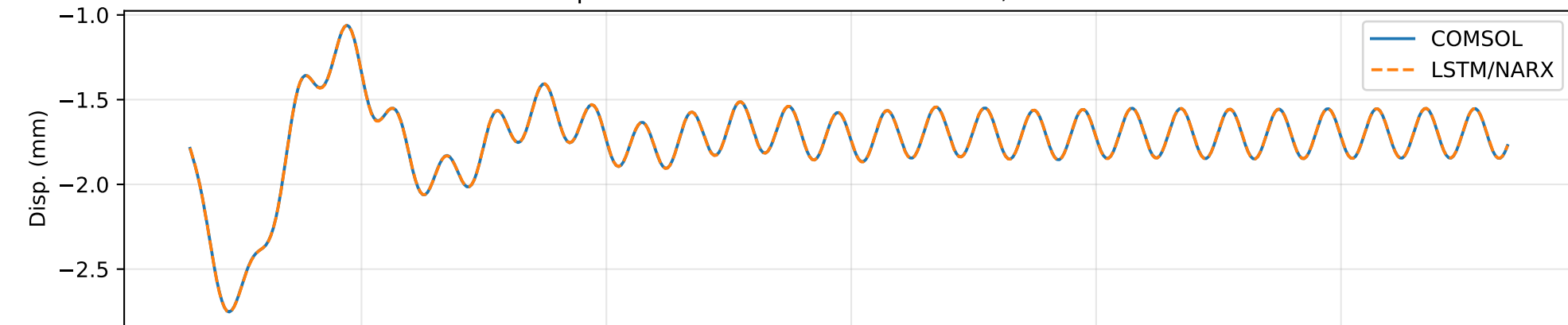
Displacement: RMSE=0.001251 mm, R2=1.0000
