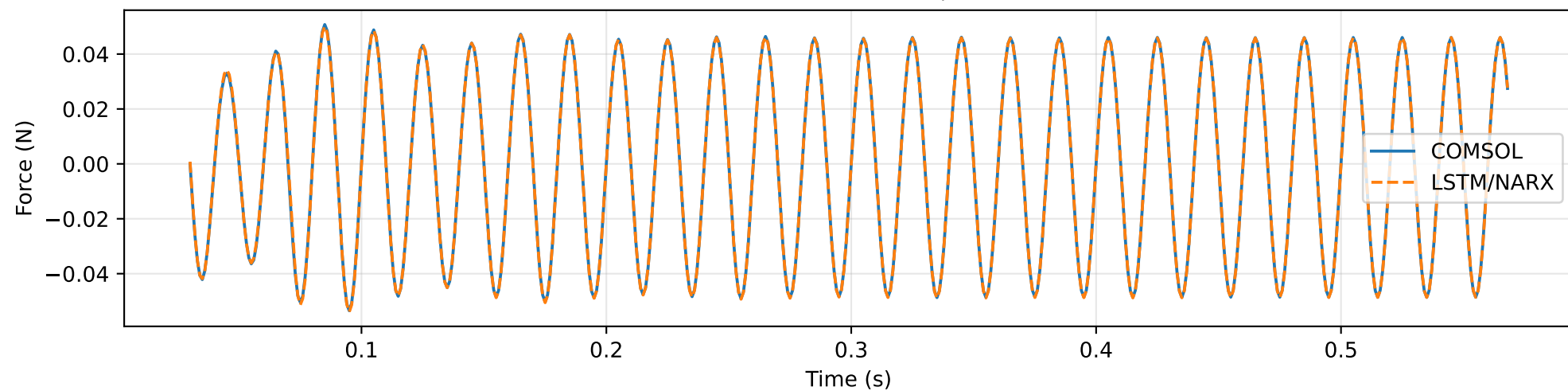
Force: RMSE=0.0002739 N, R2=0.9999
