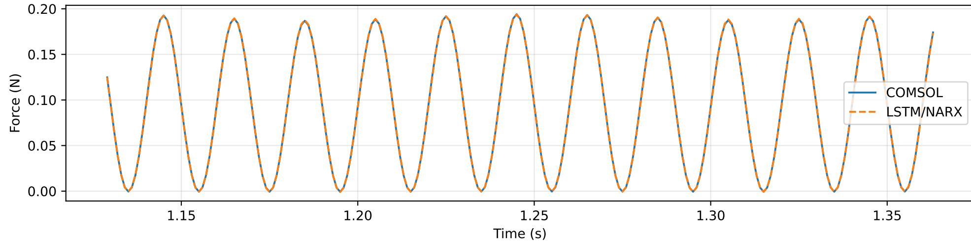
Force: RMSE=0.0005625 N, R2=0.9999
