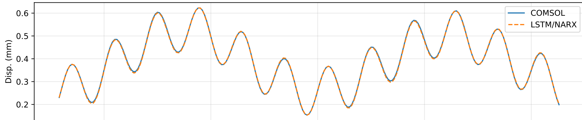
Displacement: RMSE=0.002855 mm, R2=0.9994
