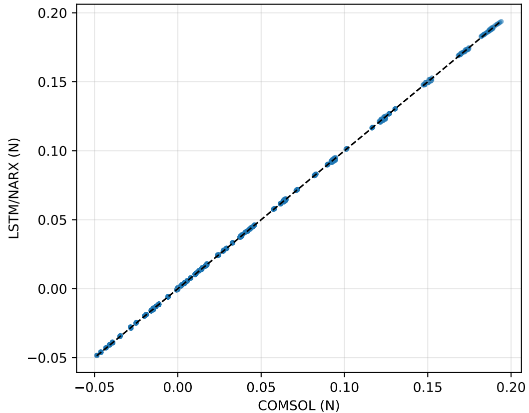
Validation: Force parity, R^2=1.0000
