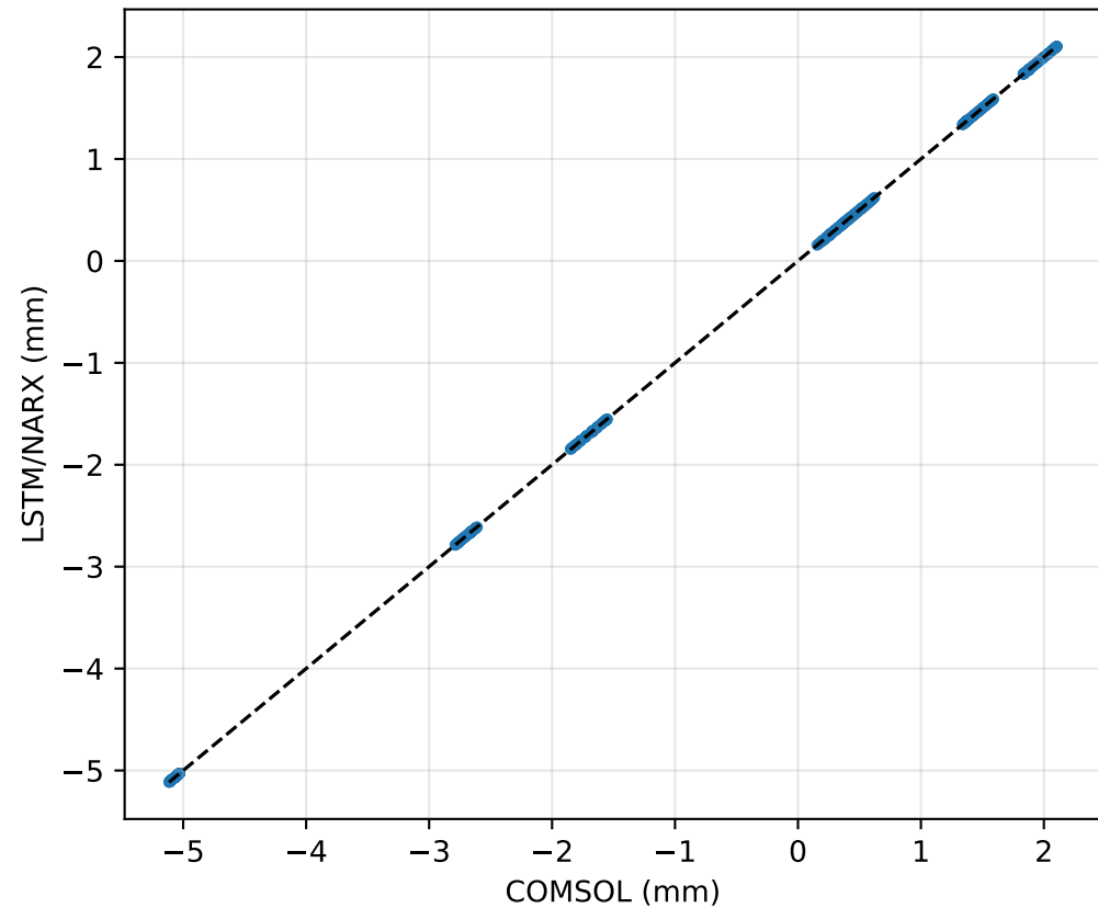
Validation: Displacement parity, R^2=1.0000
