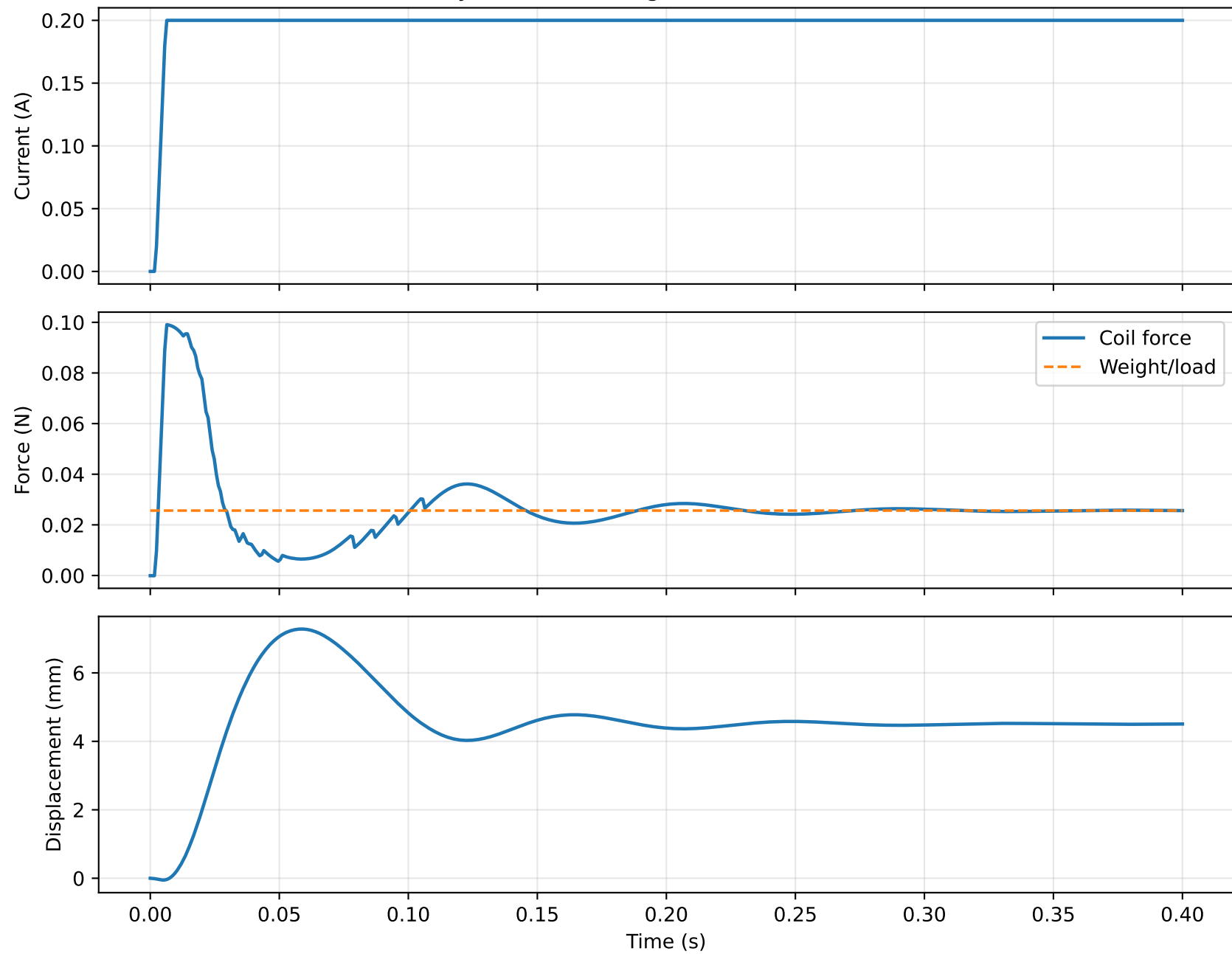
Synchronized Single Actuator Dataset
