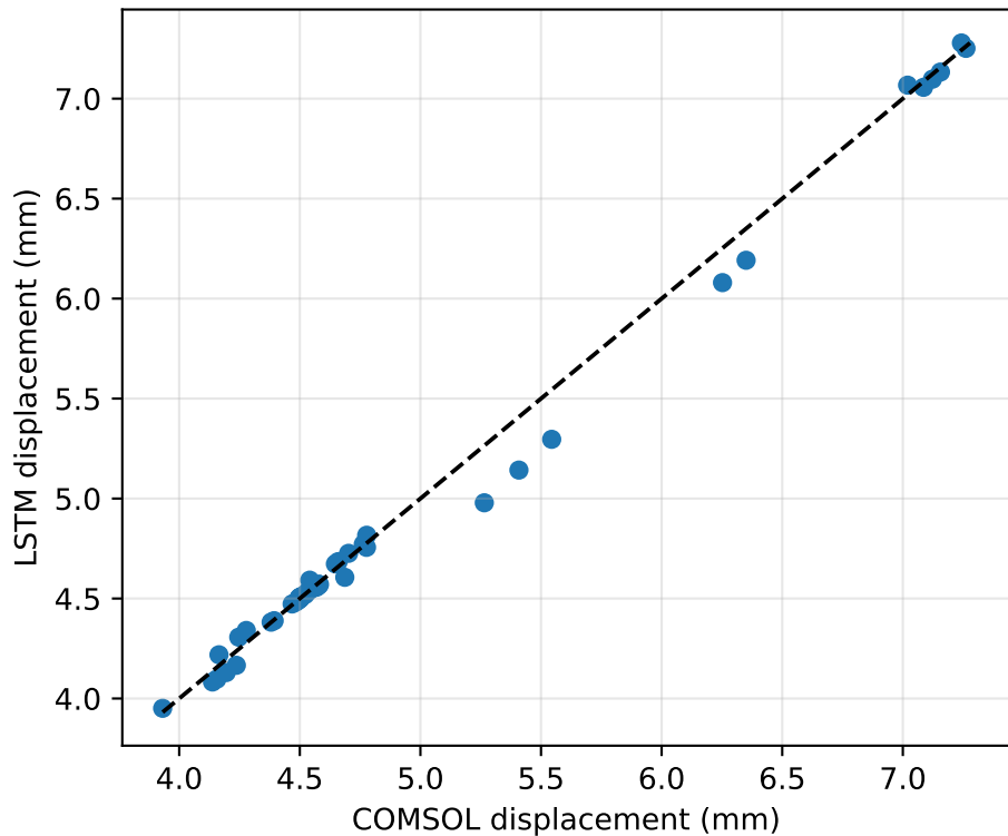
Displacement parity, R^2 = 0.9927
