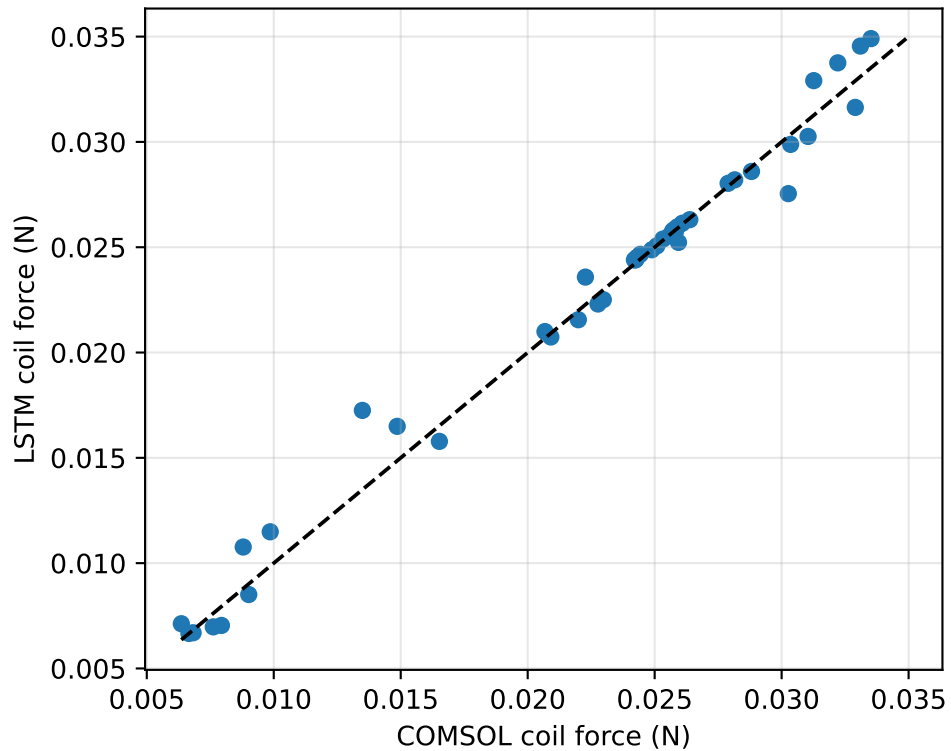
Force parity, R^2 = 0.9833
