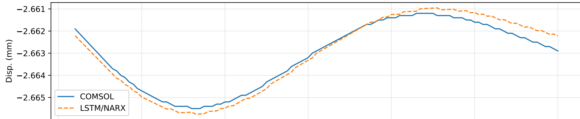
Displacement: RMSE=0.0003033 mm, R2=0.9571
