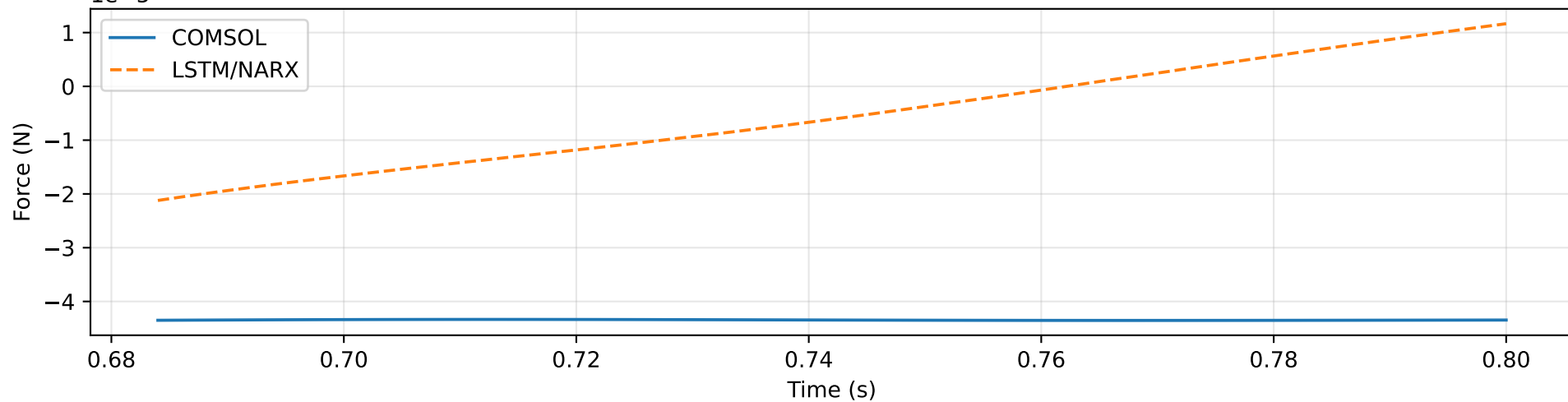
Force: RMSE=3.926e-05 N, R2=-369359.2954
