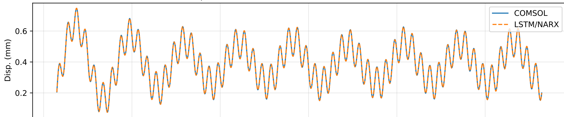
Displacement: RMSE=0.001565 mm, R2=0.9999
