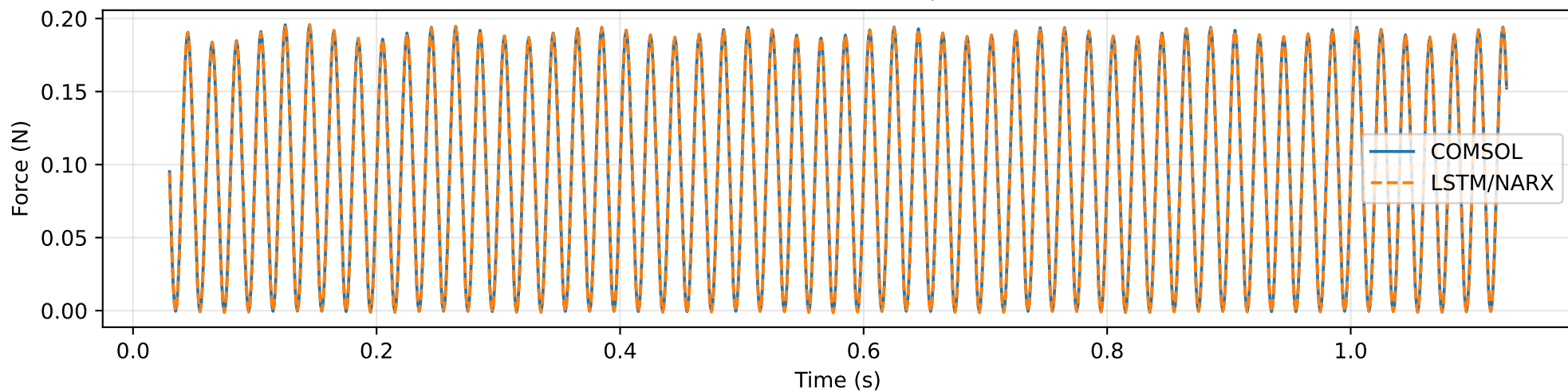
Force: RMSE=0.0003471 N, R2=1.0000
