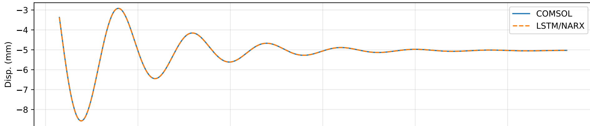
Displacement: RMSE=0.0007322 mm, R2=1.0000
