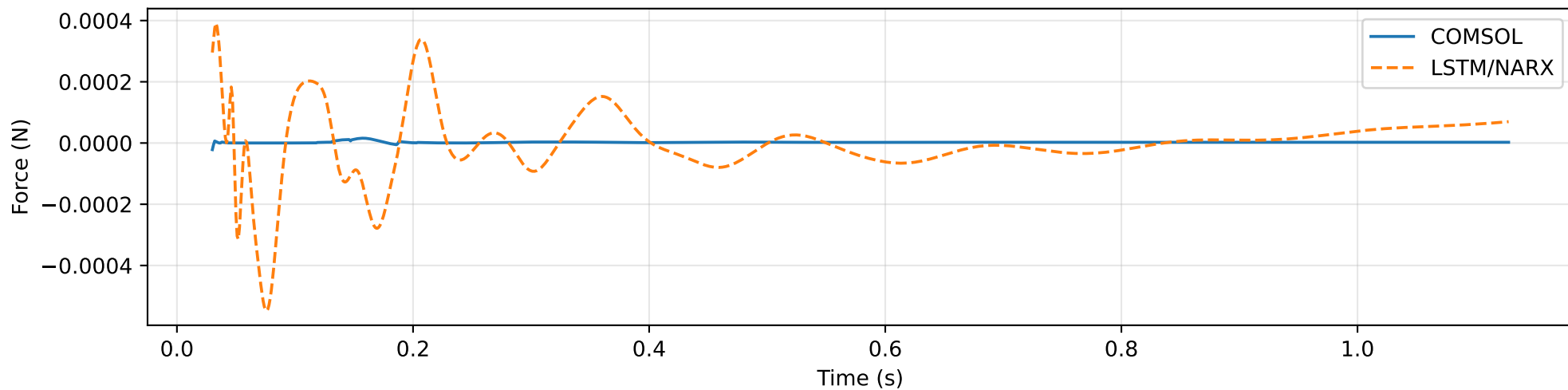
Force: RMSE=0.0001069 N, R2=-2332.1744
