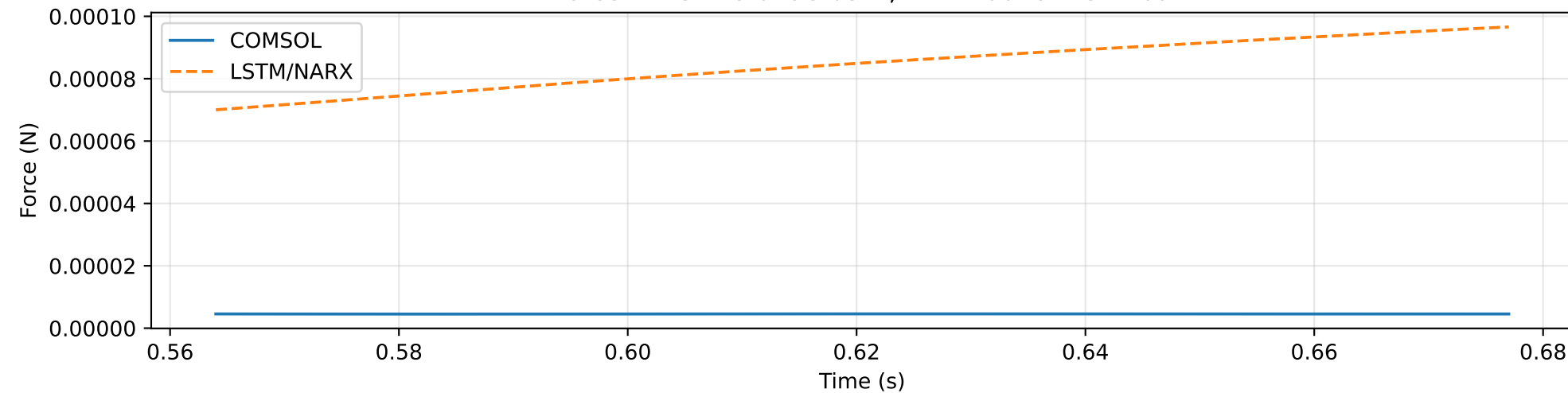
Force: RMSE=8.019e-05 N, R2=-19979478.2469
