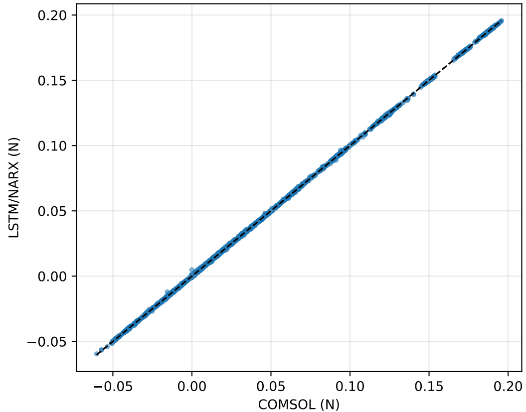
Train: Force parity, R^2=1.0000
