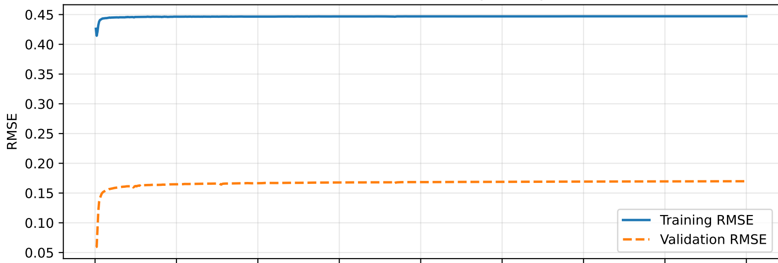
Enhanced LSTM Training History
