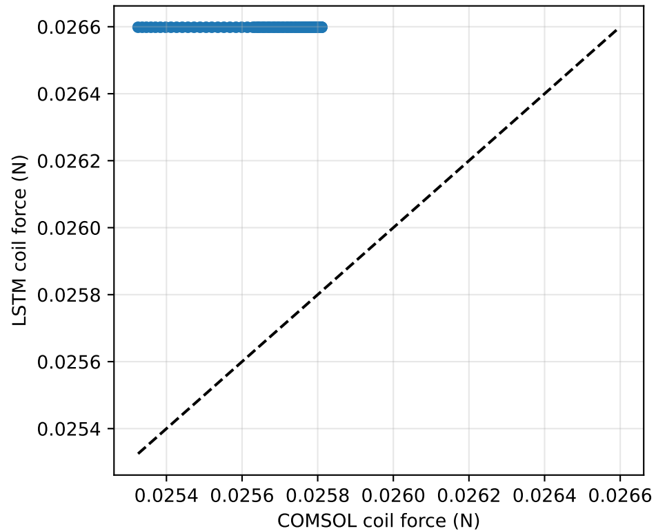
Force parity, R^2 = -43.0848
