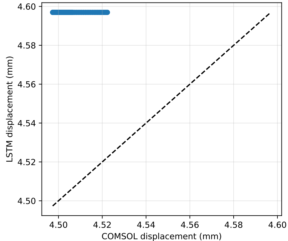
Displacement parity, R^2 = -158.1297
