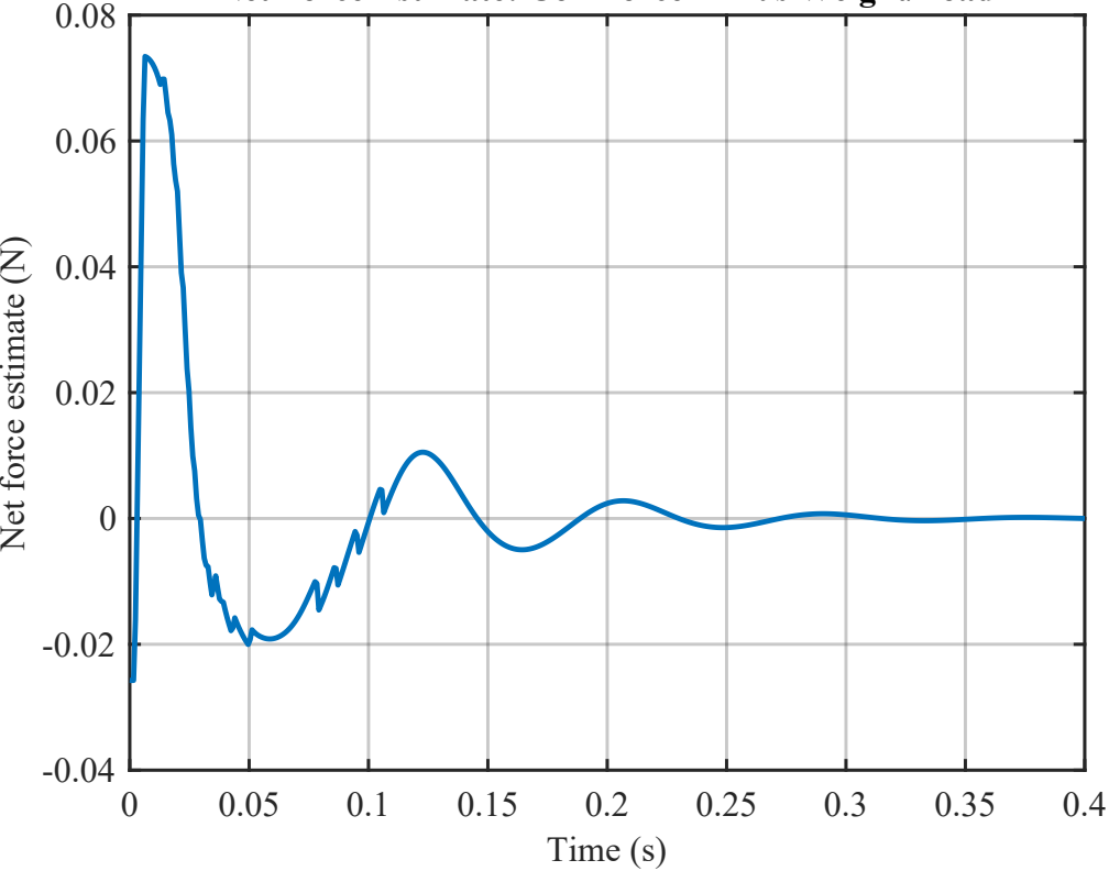
Net Force Estimate: Coil Force Minus Weight/Load
