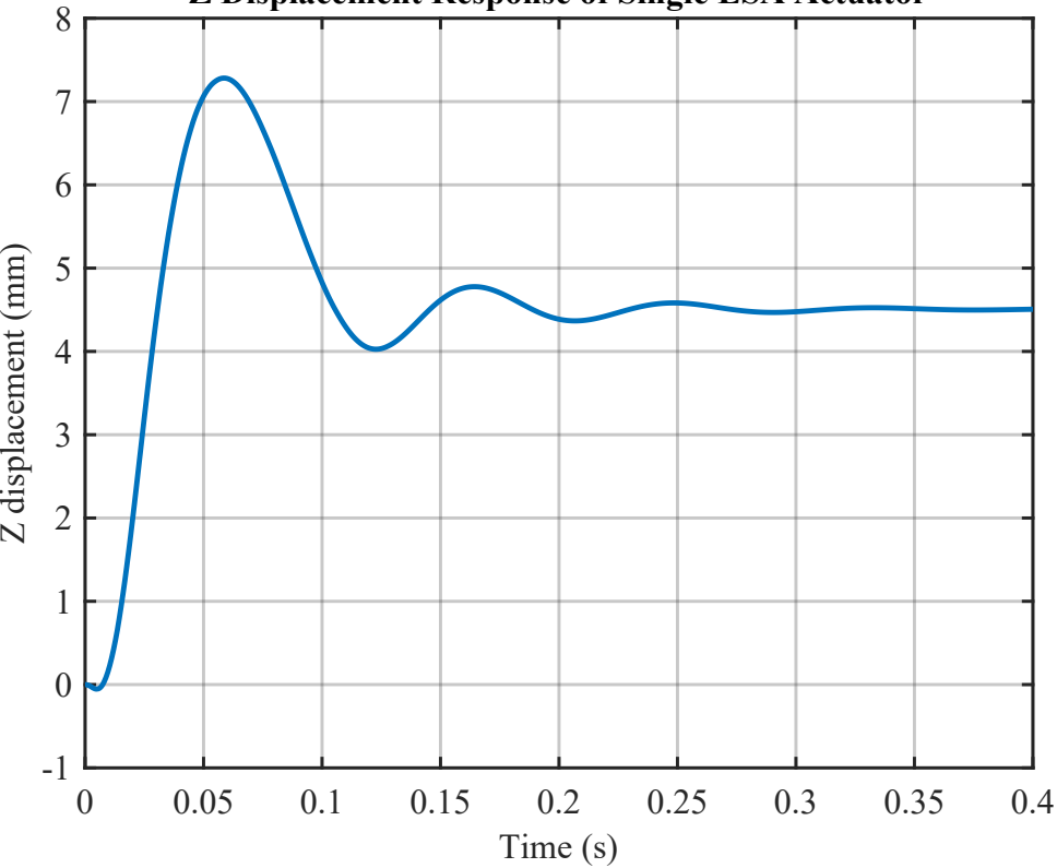
Z Displacement Response of Single ESA Actuator
