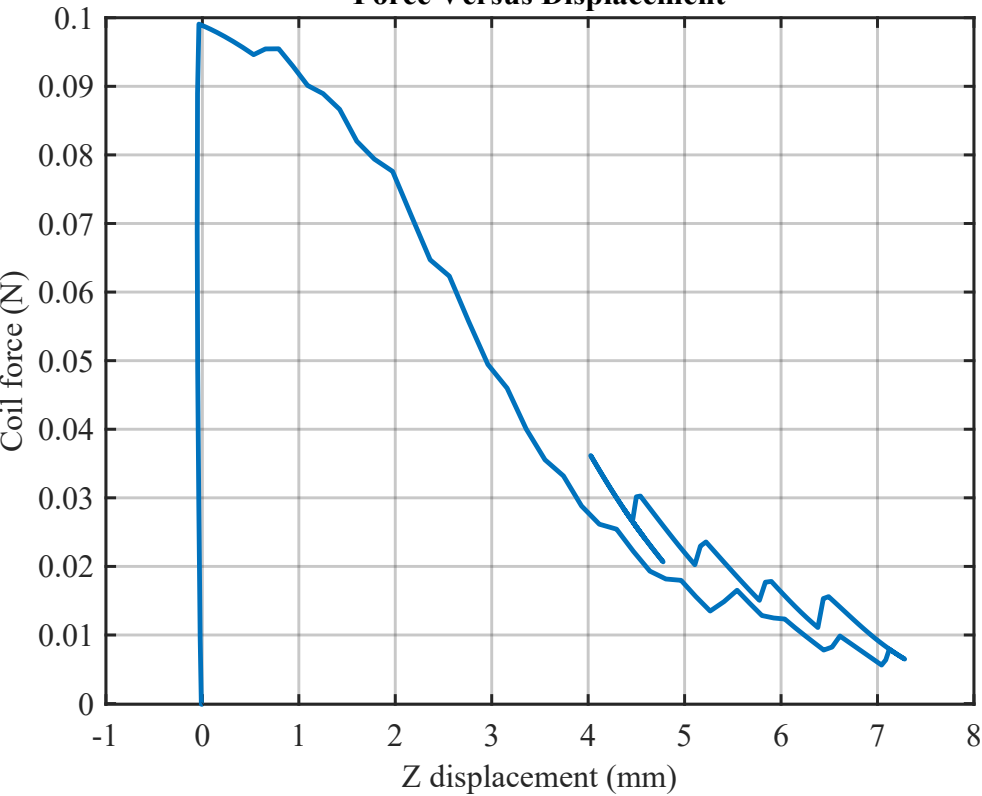
Force Versus Displacement
