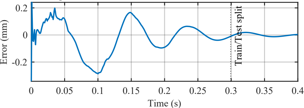
Displacement Prediction Error: COMSOL minus LSTM
