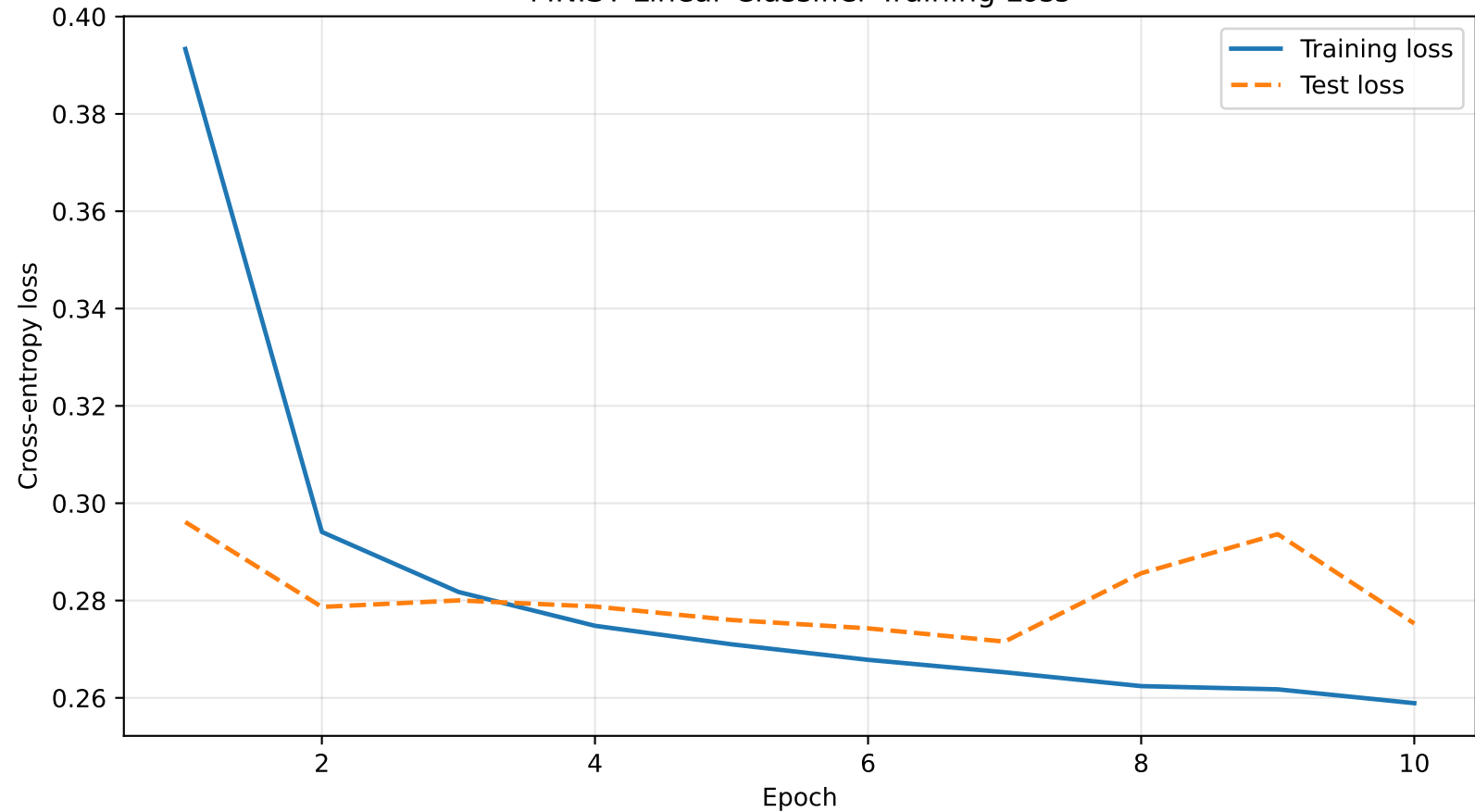
MNIST Linear Classifier Training Loss
