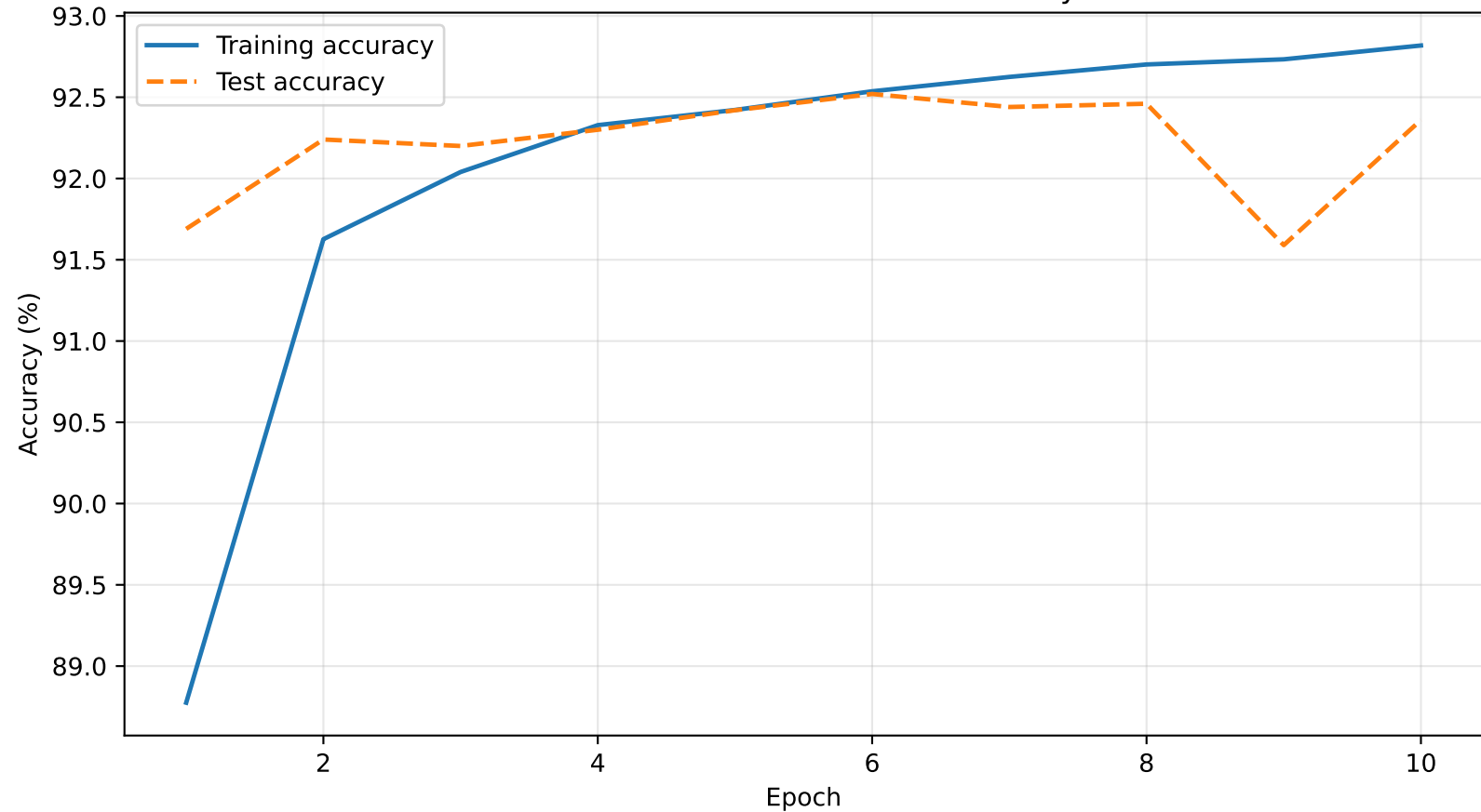
MNIST Linear Classification Accuracy
