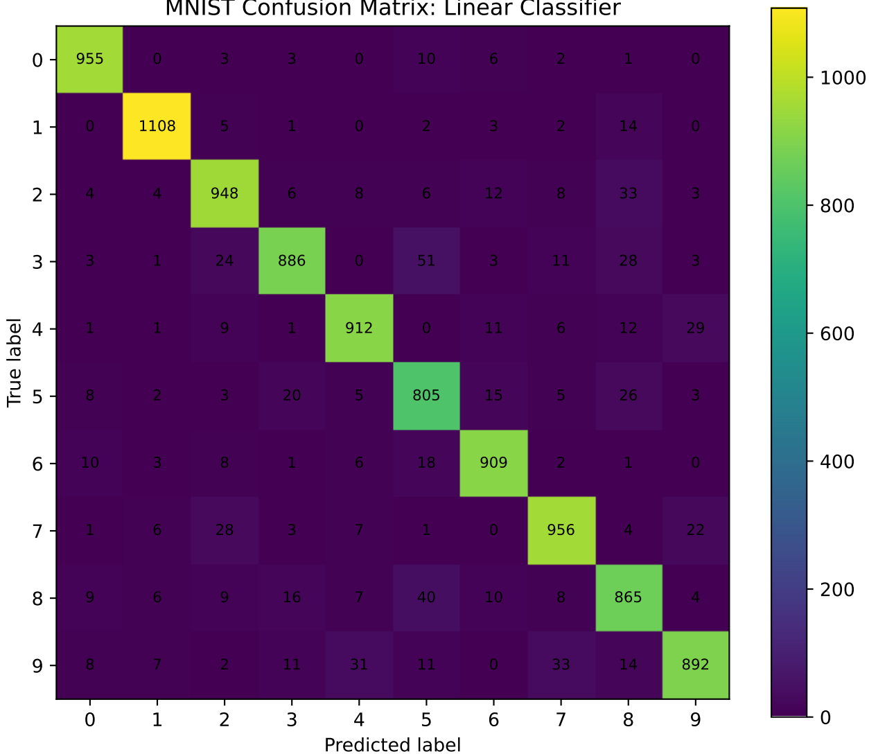
MNIST Confusion Matrix: Linear Classifier
