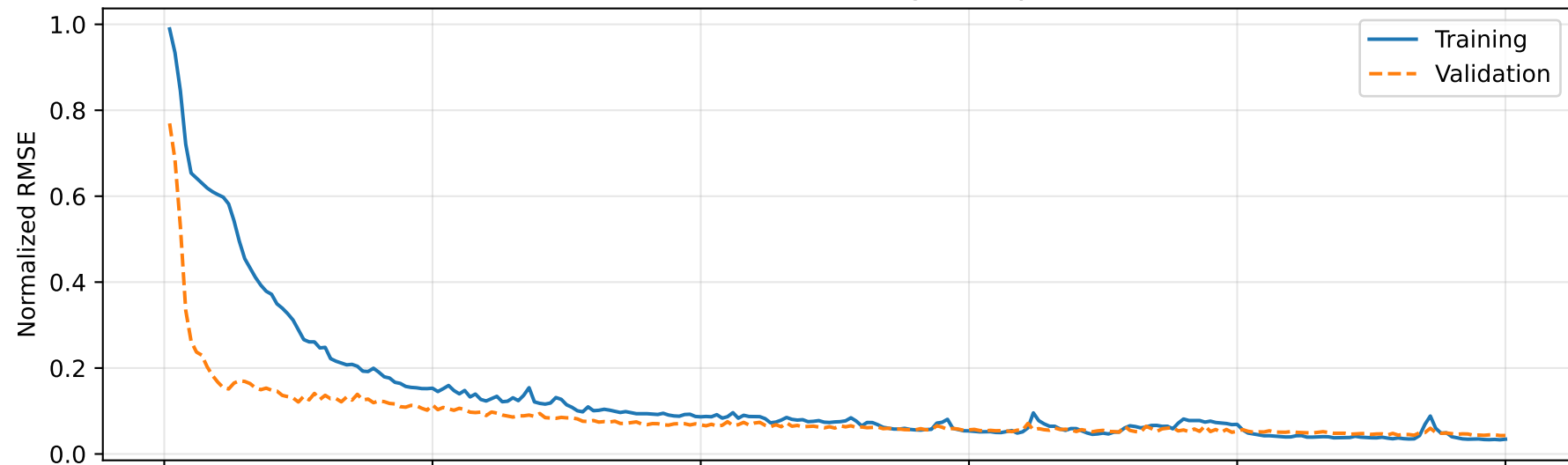
LSTM/NARX Training History
