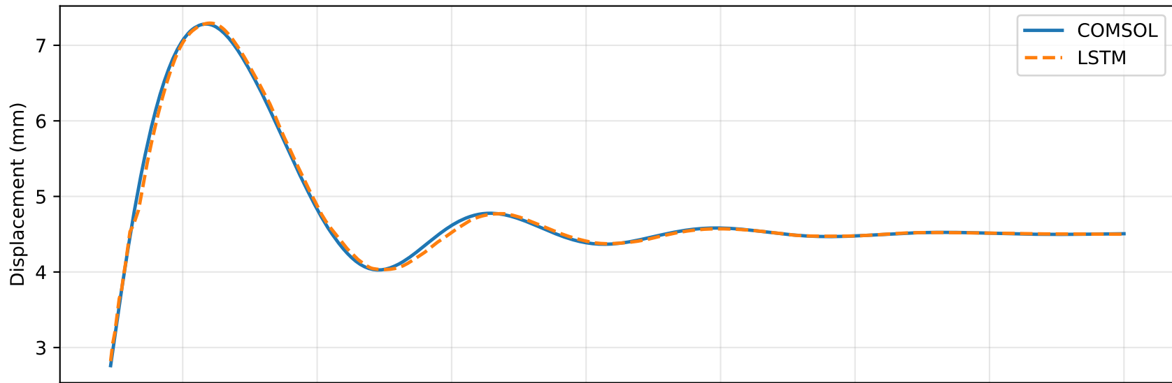
Displacement Prediction, test RMSE = 0.08099 mm, R2 = 0.9927
