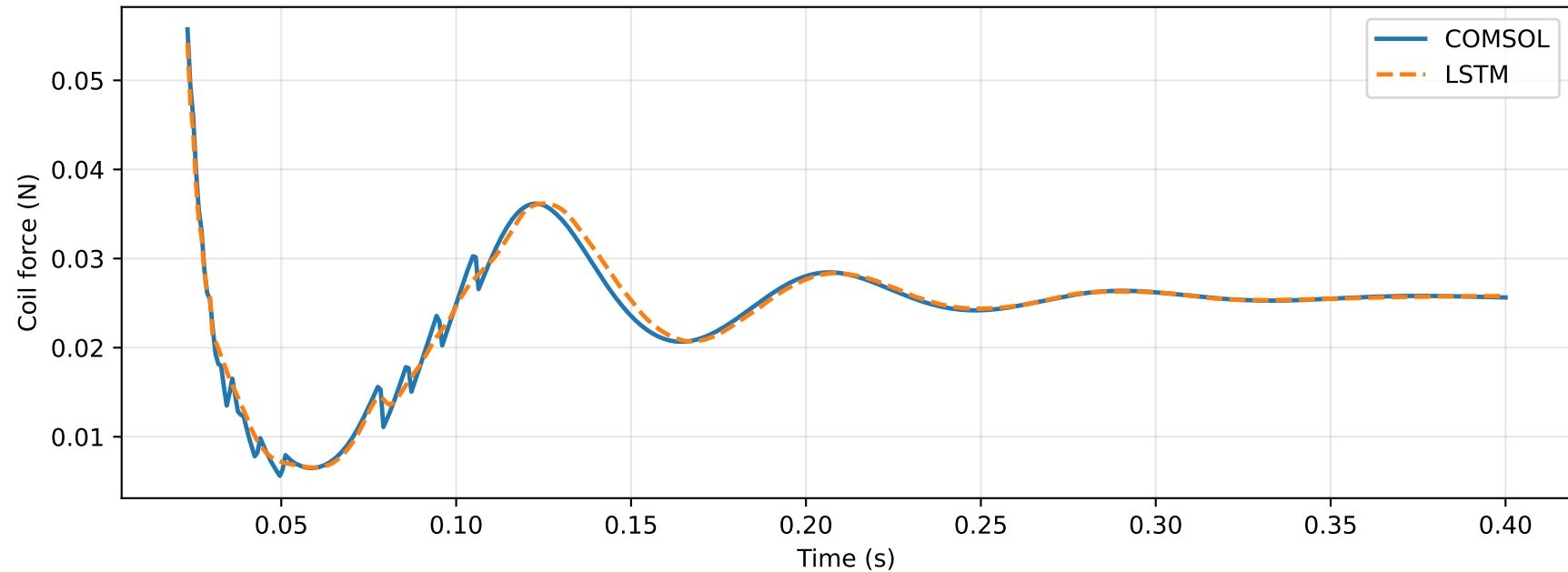
Force Prediction, test RMSE = 0.001002 N, R2 = 0.9833
