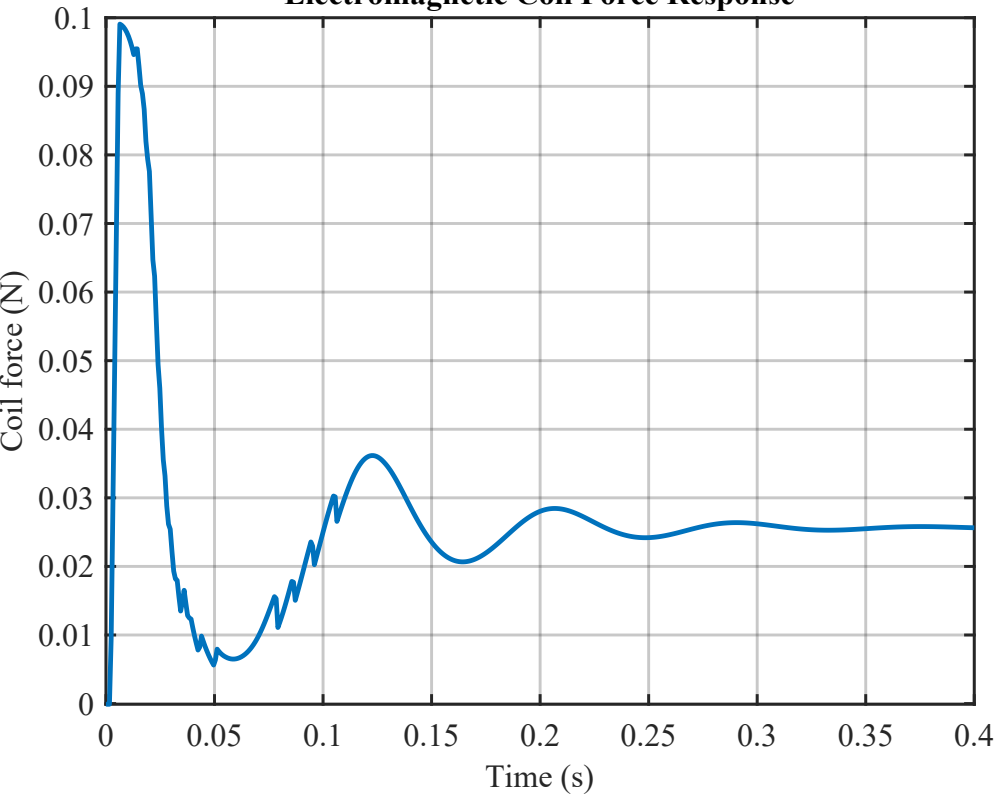
Electromagnetic Coil Force Response
