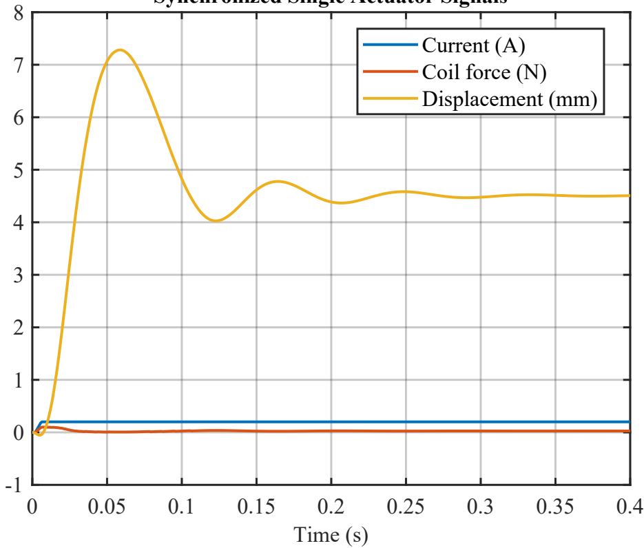
Synchronized Single Actuator Signals
