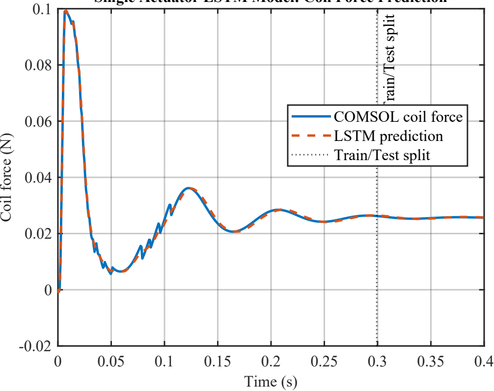
Single Actuator LSTM Model: Coil Force Prediction
