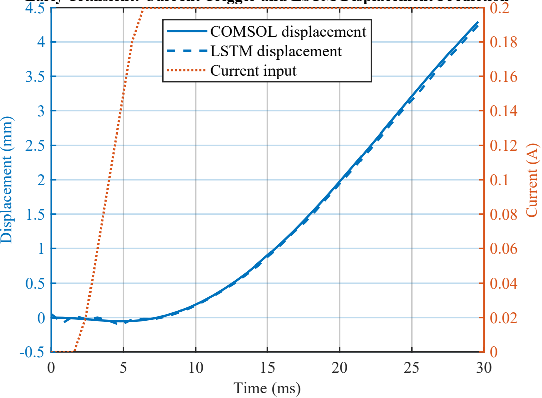
Early Transient: Current Trigger and LSTM Displacement Prediction
