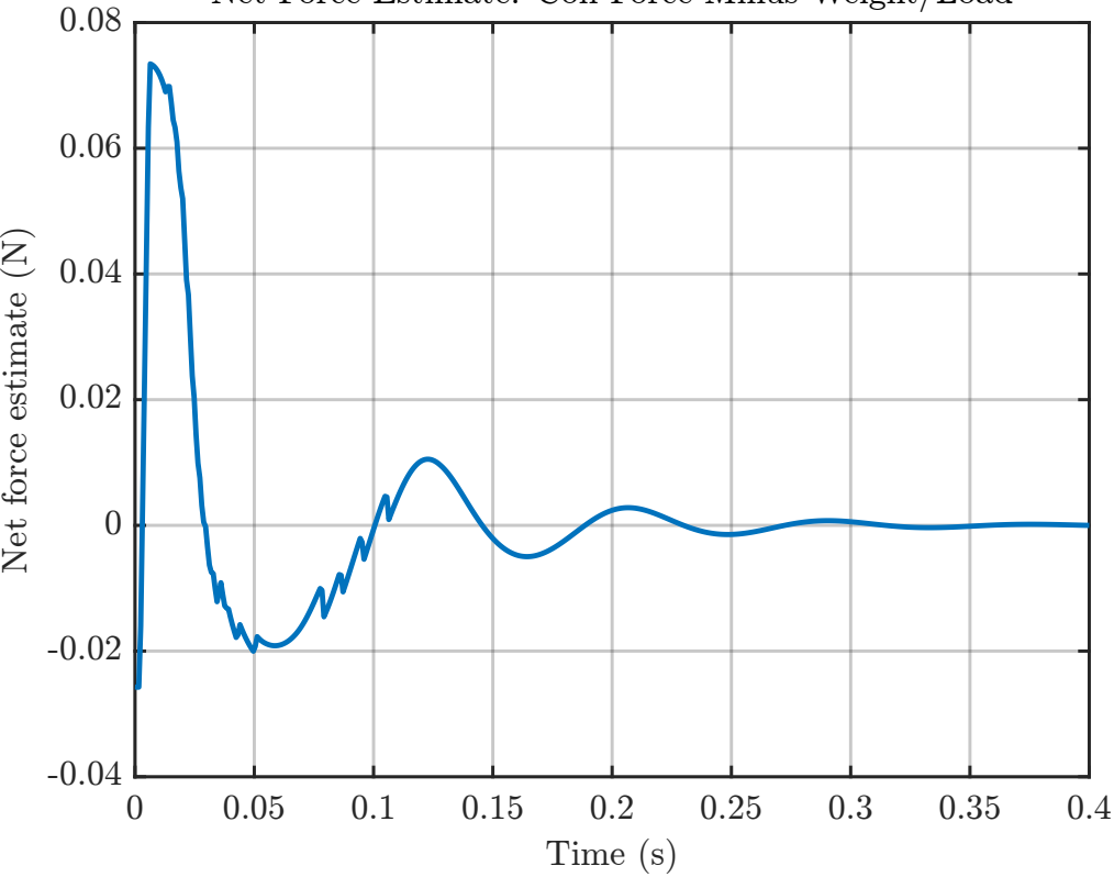
Net Force Estimate: Coil Force Minus Weight/Load
