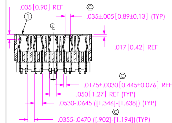
SECTION 'B'-B' SCALE 2.5:1
