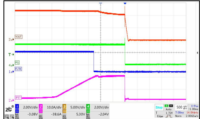
Figure 19. OCP ILIMIT=19A
