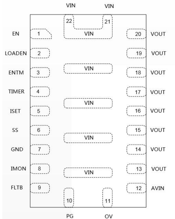
Figure 2. Top View
