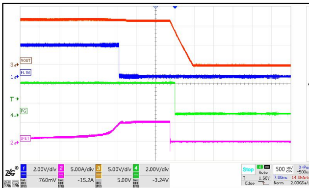
Figure 22. OCP ILIMIT=5A
