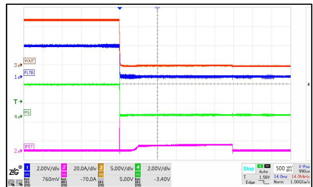
Figure 23. SCP Entry ILIMIT=5A
