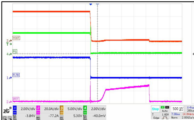
Figure 20. S_{CP} Entry ILIMIT=19A
