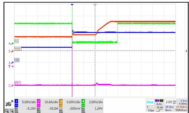
Figure 25. LINE SPIKE ILIMIT=19A
