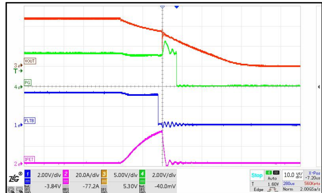
Figure 21. S_{CP} Entry Detail ILIMIT=19A
