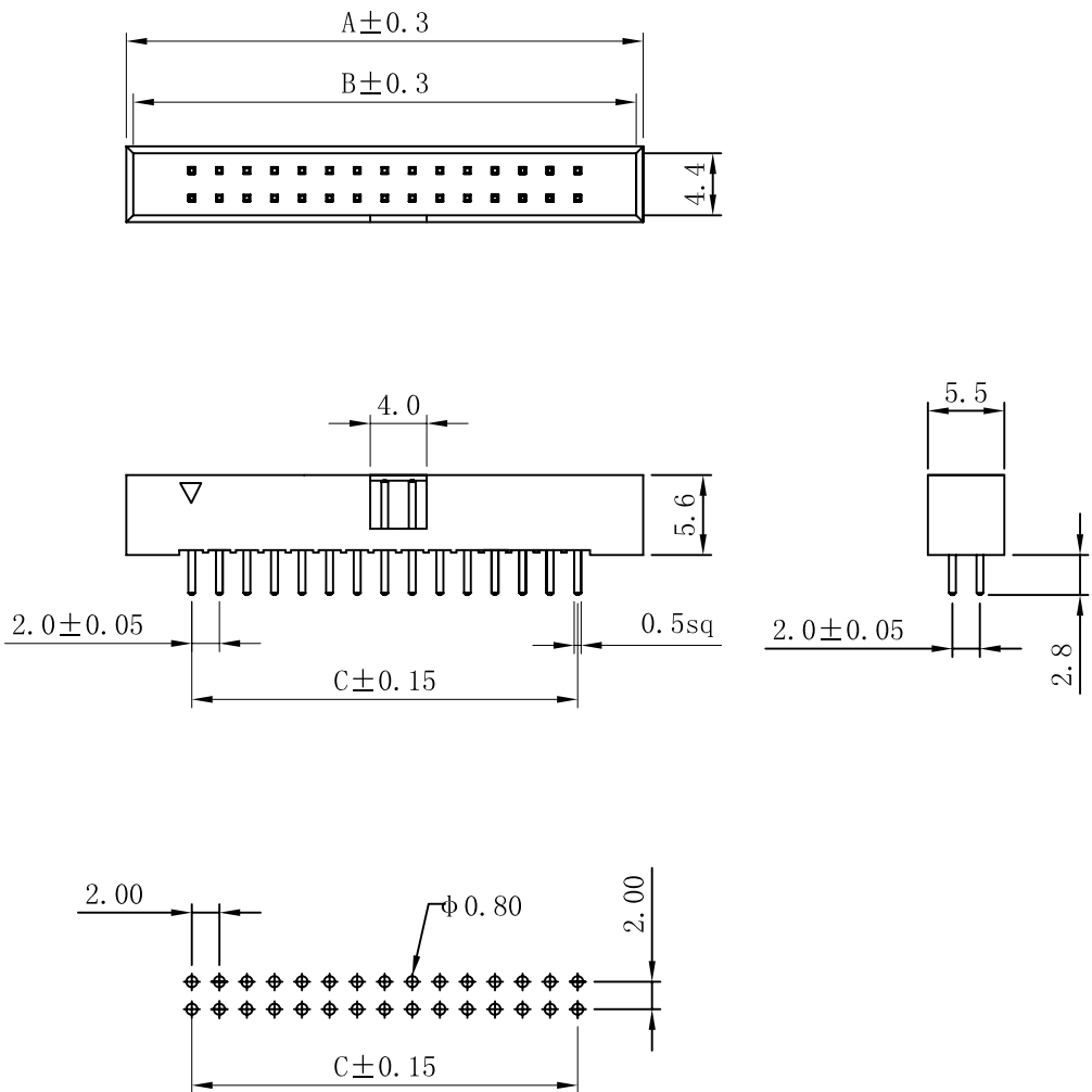
PCB LAYOUT
