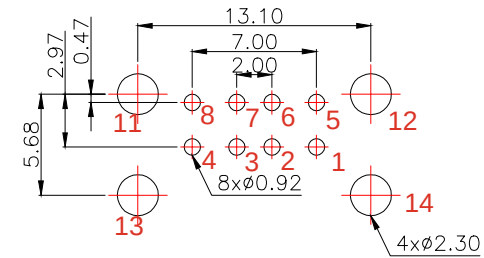
PCB.WELDING DRAWING (TOLERANCE:±0.05)
