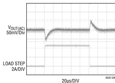
1.2V Single Phase Output Load Transient Response
