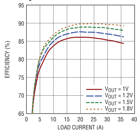
Dual Phase Single Output Efficiency vs Output Current, V_{IN} = 12V , f_s = 450kHz
