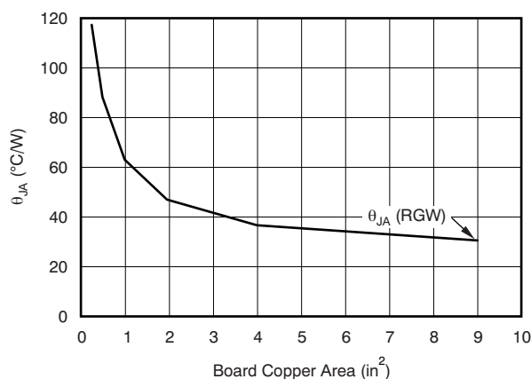
Figure 53. \theta_{JA} versus Board Size
