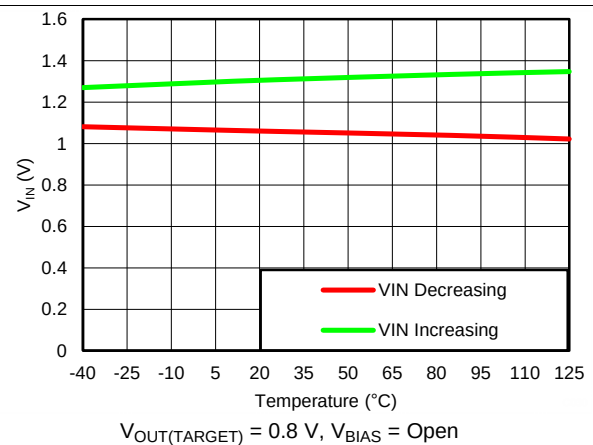
Figure 30. Minimum ANY-OUT V_{OUT} , No BIAS Input UVLO Threshold vs Temperature
