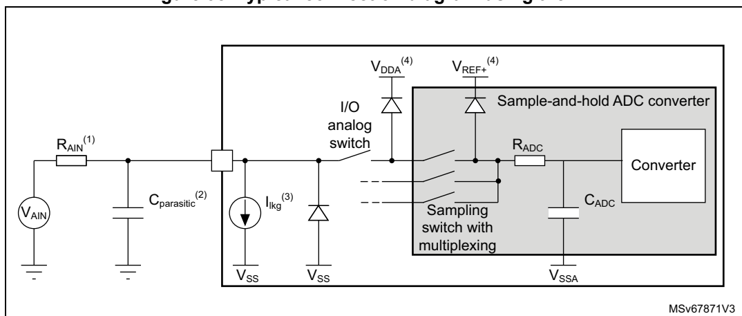
Figure 38. Typical connection diagram using the ADC
