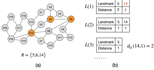
Figure 1. An explanation of distance labeling: (a) an example graph G , (b) Compute a label L(v) for each vertex v \in V in G in advance.
