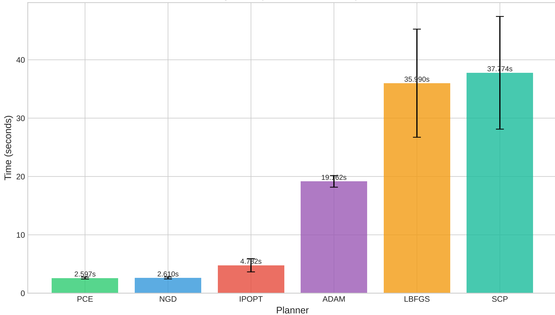
Average Computation Time Comparison
