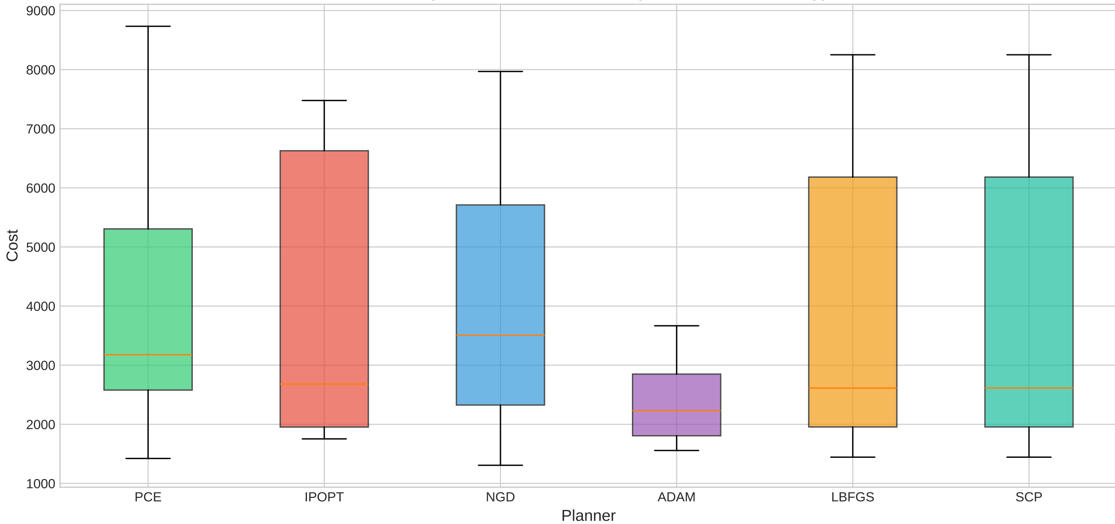
Cost Comparison Across Planners (Successful Runs Only)
