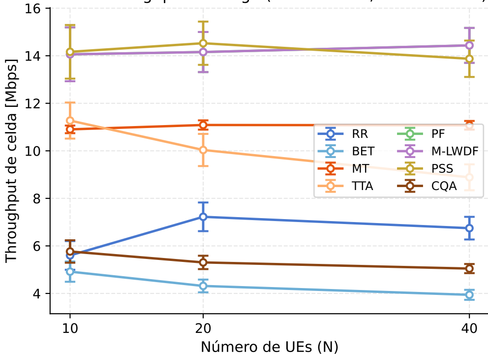
F1 — Throughput vs carga (D1 uniforme, T1 full-buffer)
