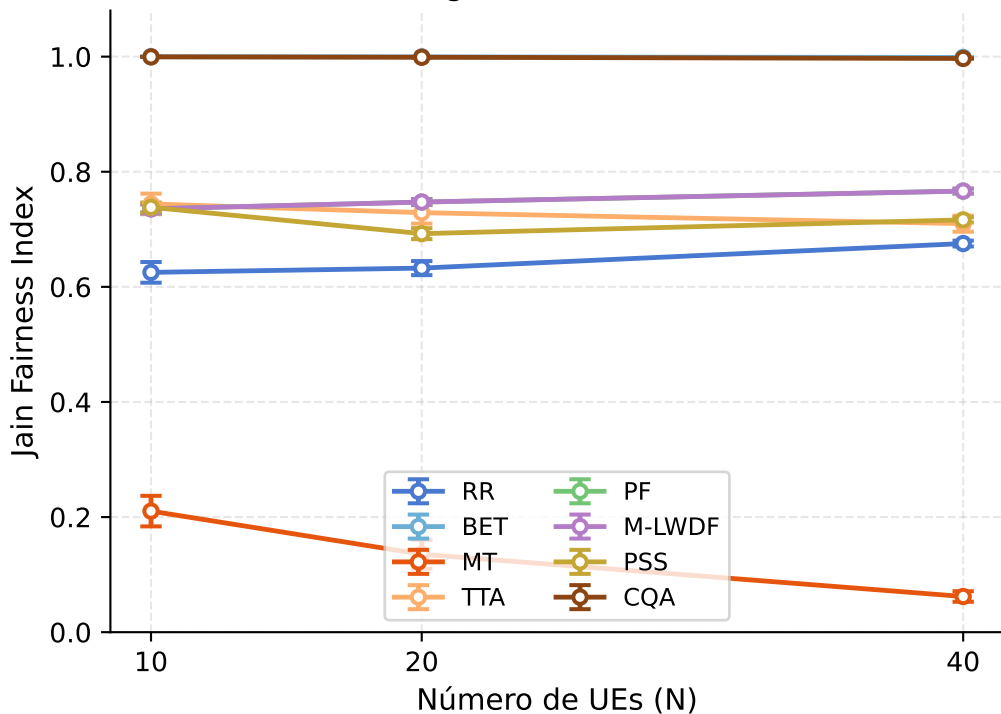
F3 — Fairness vs carga (D2 clusterizado, T1 full-buffer)
