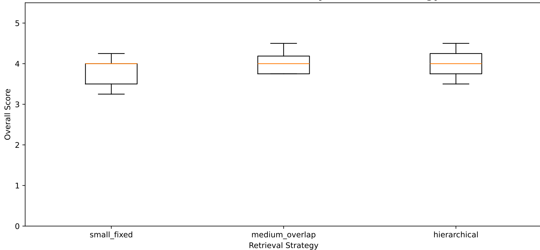
Distribution of Overall Scores by Retrieval Strategy
